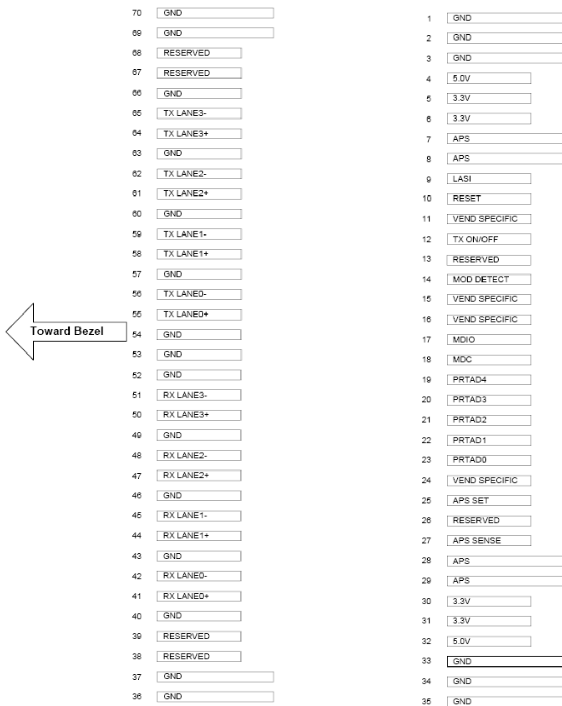
Figure2.Electrical Pin-out Details
