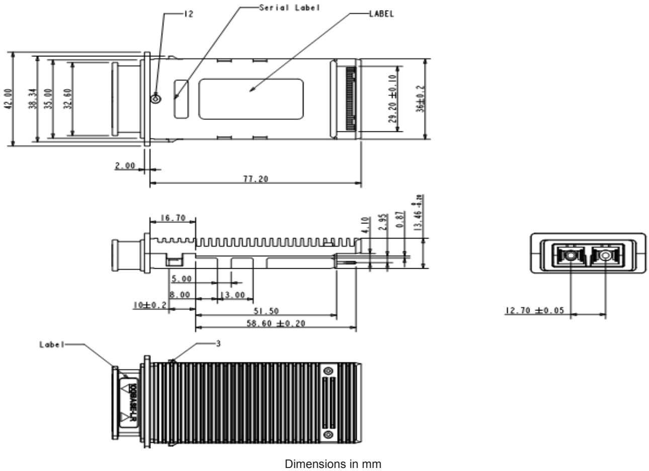
Figure3. Mechanical Dimensions
